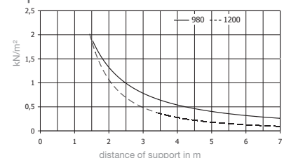
Span chart
