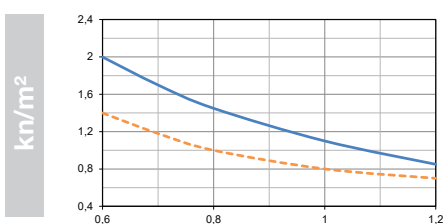
distance A in m — wind pressure - snow at 15° roof pitch - - - wind suction
