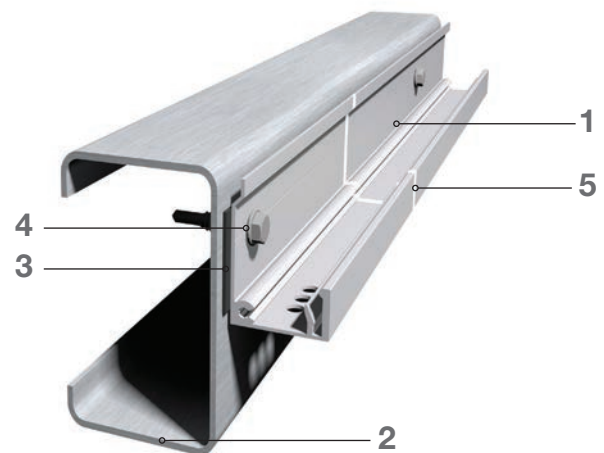
Montage in Laibung (Abb. 2)
